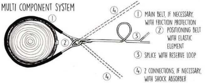
Figure 9: Connection of multi-component system
