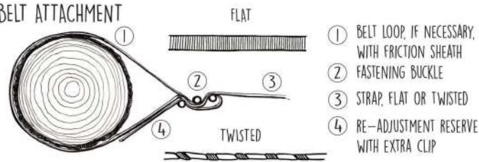
Figure 10: Connection of belt
