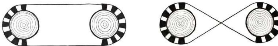
Figure 16: Recommended ways of installing the cable-and-slat system
