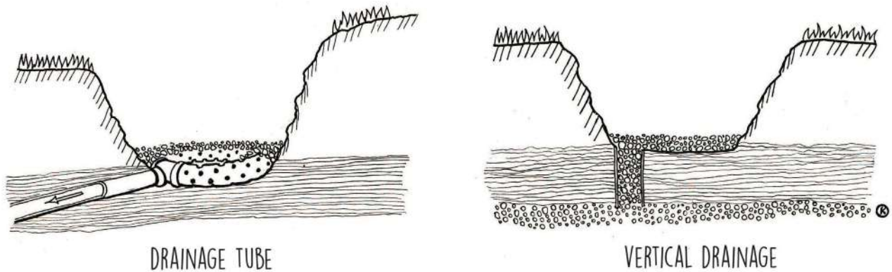
Figure 16: Various types of drainage systems in the planting pit.
